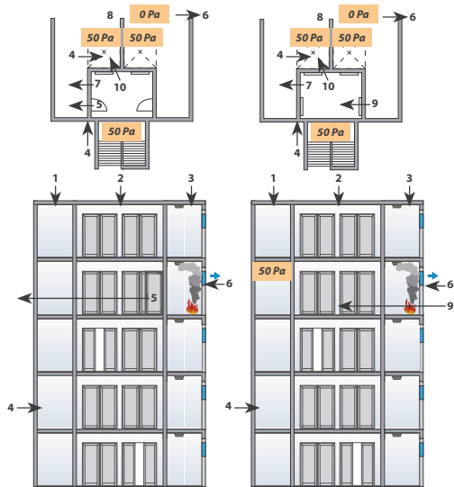
1. Staircase. / 2. Lobby. / 3. Living quarters. / 4. External air supply. / 5. Door gratings, etc. / 6. Air exhaust. / 7. Overpressure damper for discharging air to the exterior. / 8. Living quarters. / 9. Lift landing. / 10. Lift cabin.
