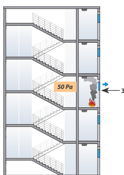
DIFFERENTIAL PRESSURE CRITERION (all the doors closed)
